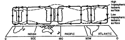
Figure 12.7 Schematic view of the east-west Walker circulation along the equator, indicating low-level convergence in regions of convection where mean upward motion occurs. (From Webster, 1987. © John Wiley & Sons, Inc. Reprinted with permission.)
