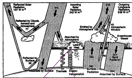
Fig. 2.30a (Kiehl and Trenberth, 1991) Annual mean global energy balance for the Earth. Units are \text{W m}^{-2} . Water condenses here Water evaporates here
